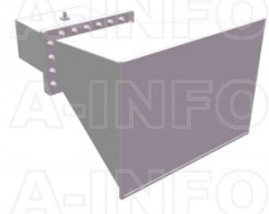
LB-1150-10-C-NFSPPO Standard Gain Horn Antenna 0.64-0.96GHz 10dB Gain N Type Female
